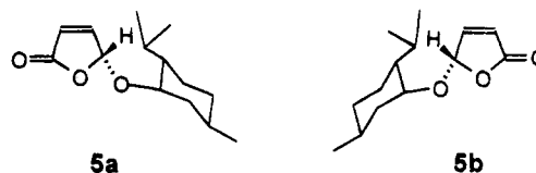
(5R)-(-)menthyloxy-2(5H)-furanone (5S)-(d)menthyloxy-2(5H)-furanone
